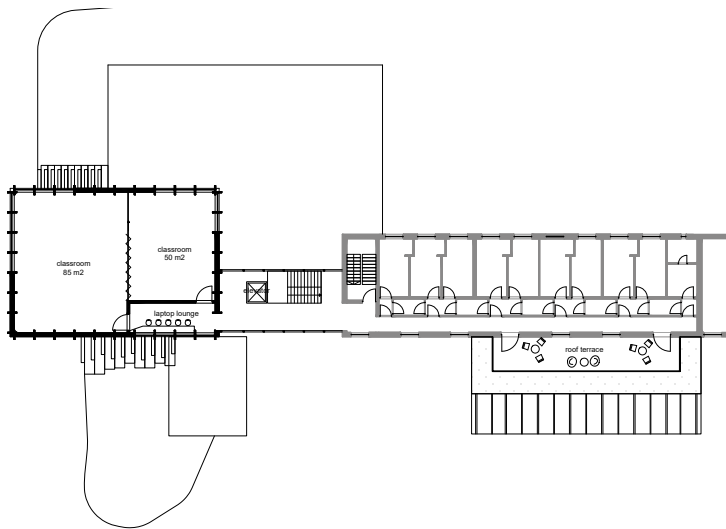
PLAN OVERETAGE 1:200
