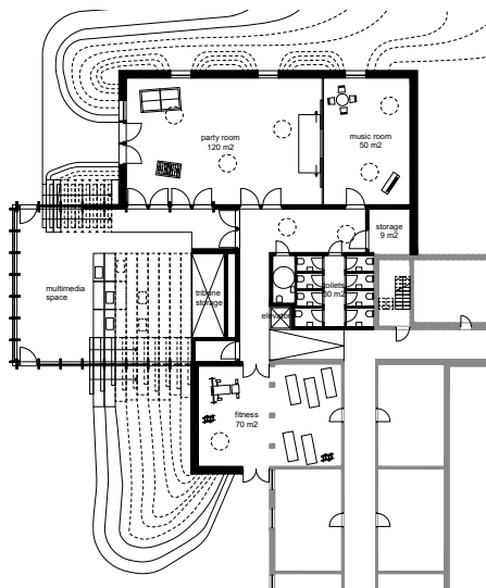
PLAN UNDERETAGE 1:200
