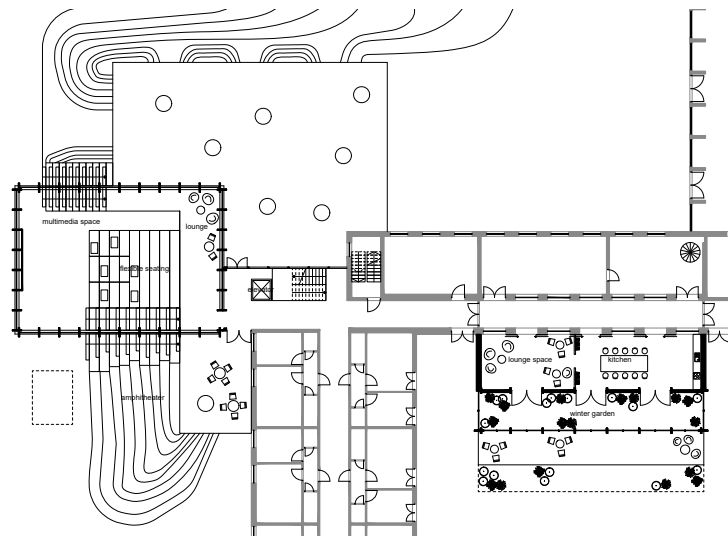
PLAN STUEETAGE 1:200
