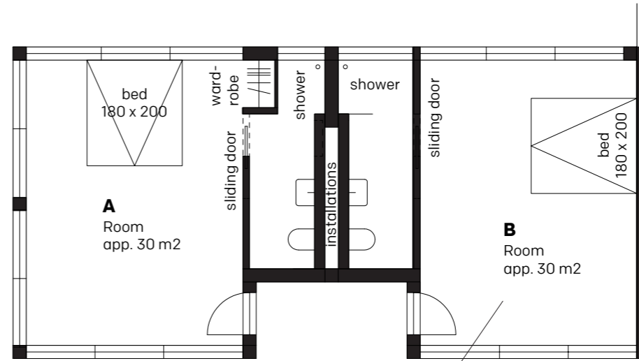
Examples of plan segments 1:100
