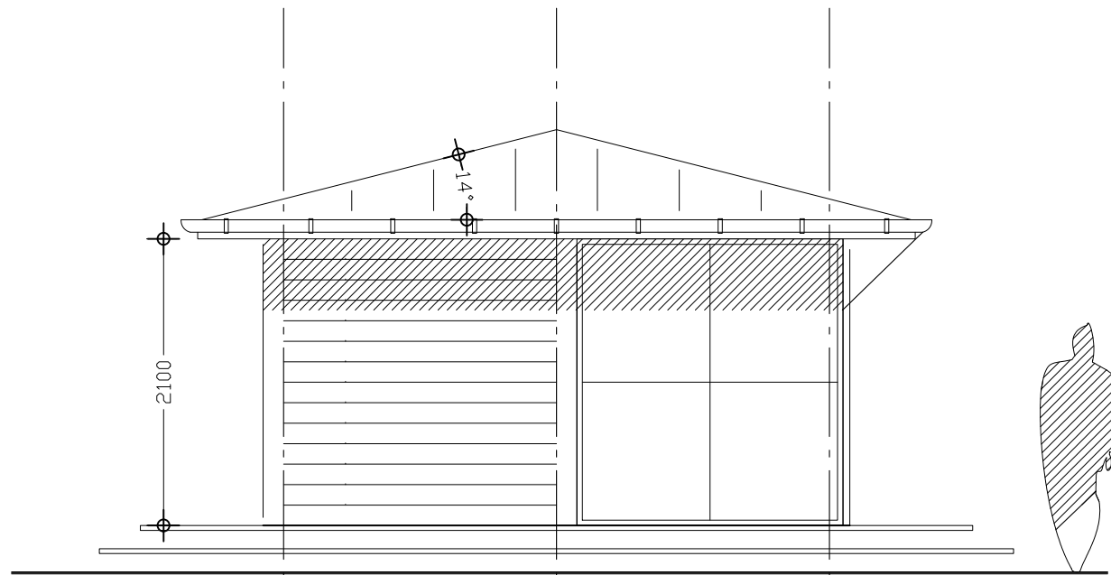
Vest facade
